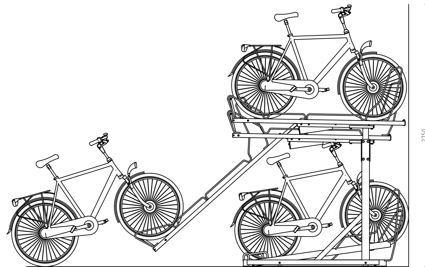
Side View
