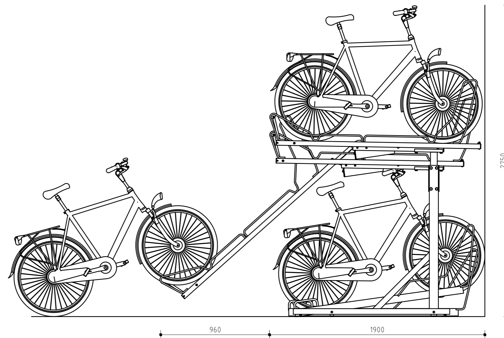
Side View
