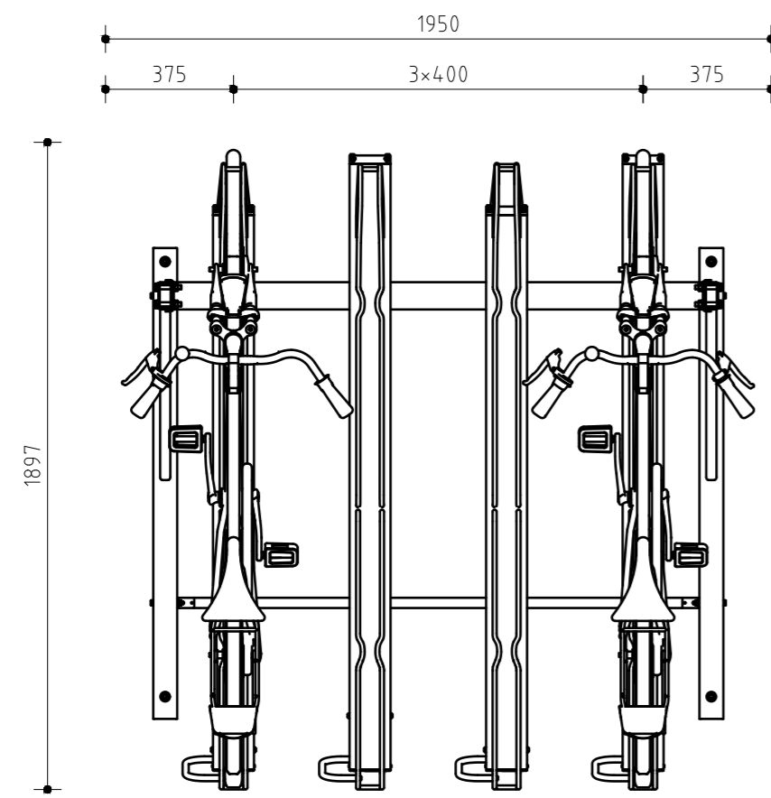
Top View
