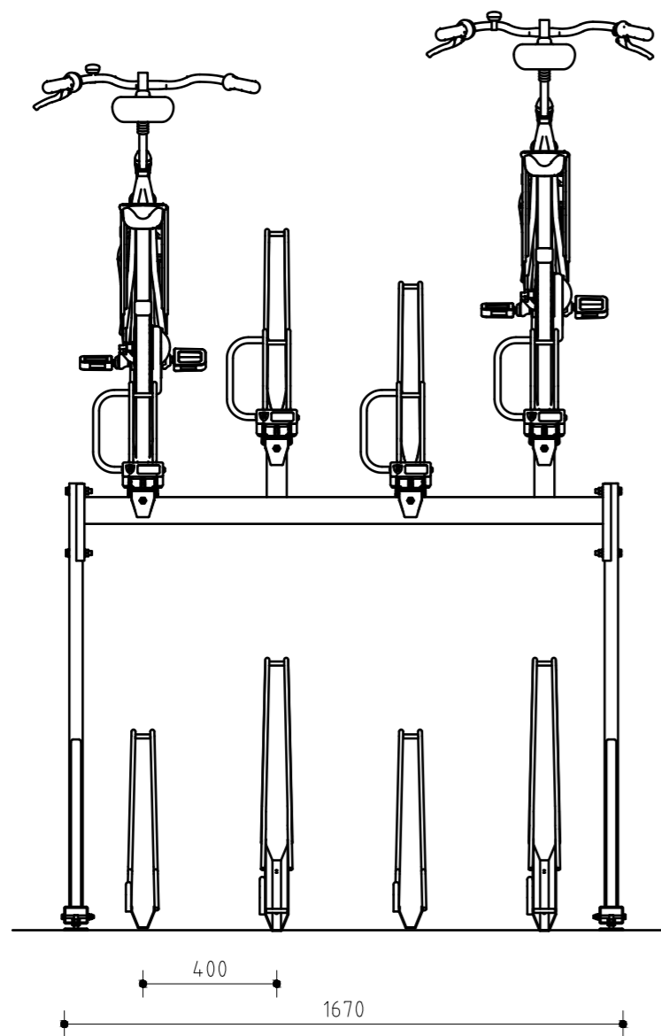
Front View
