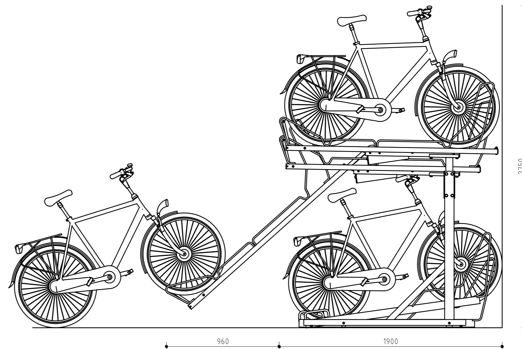
Side View
