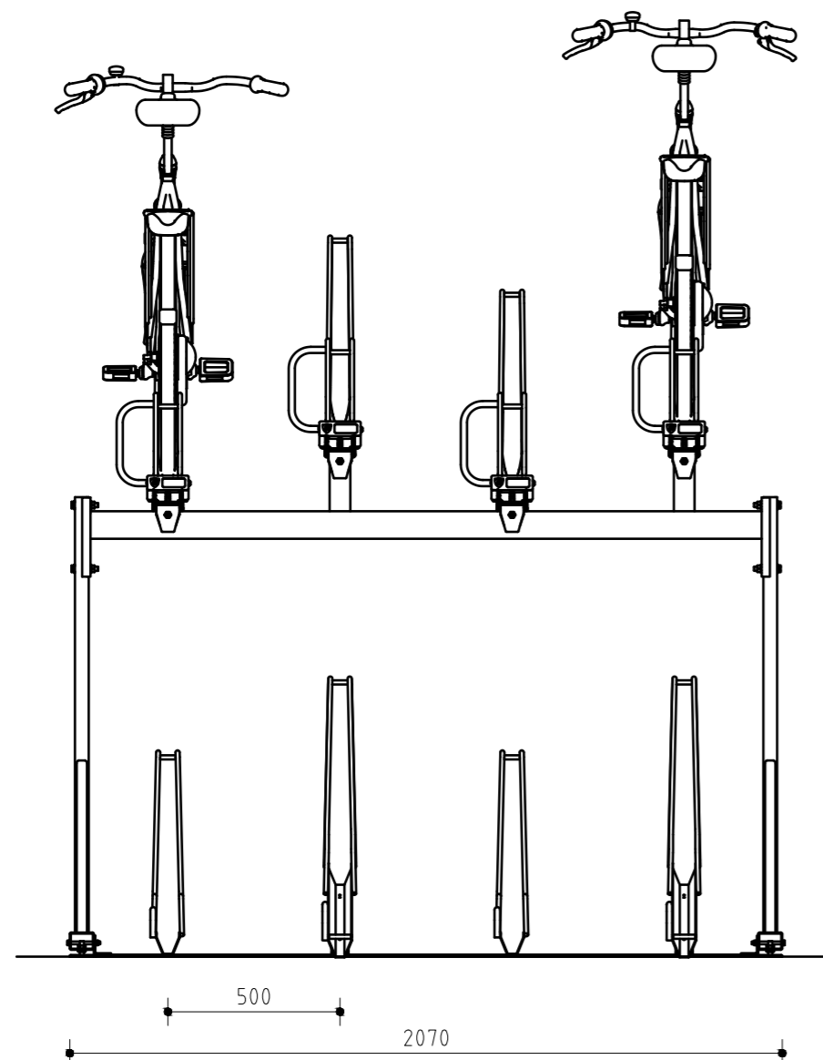
Front View
